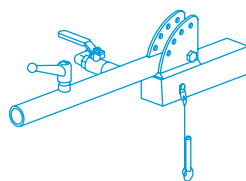
Trautman Tech Drape Forming Pipe Holder
